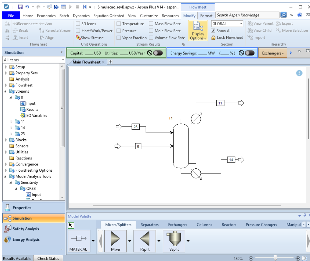
Figura 1: Fluxograma configurado no Aspen Plus
